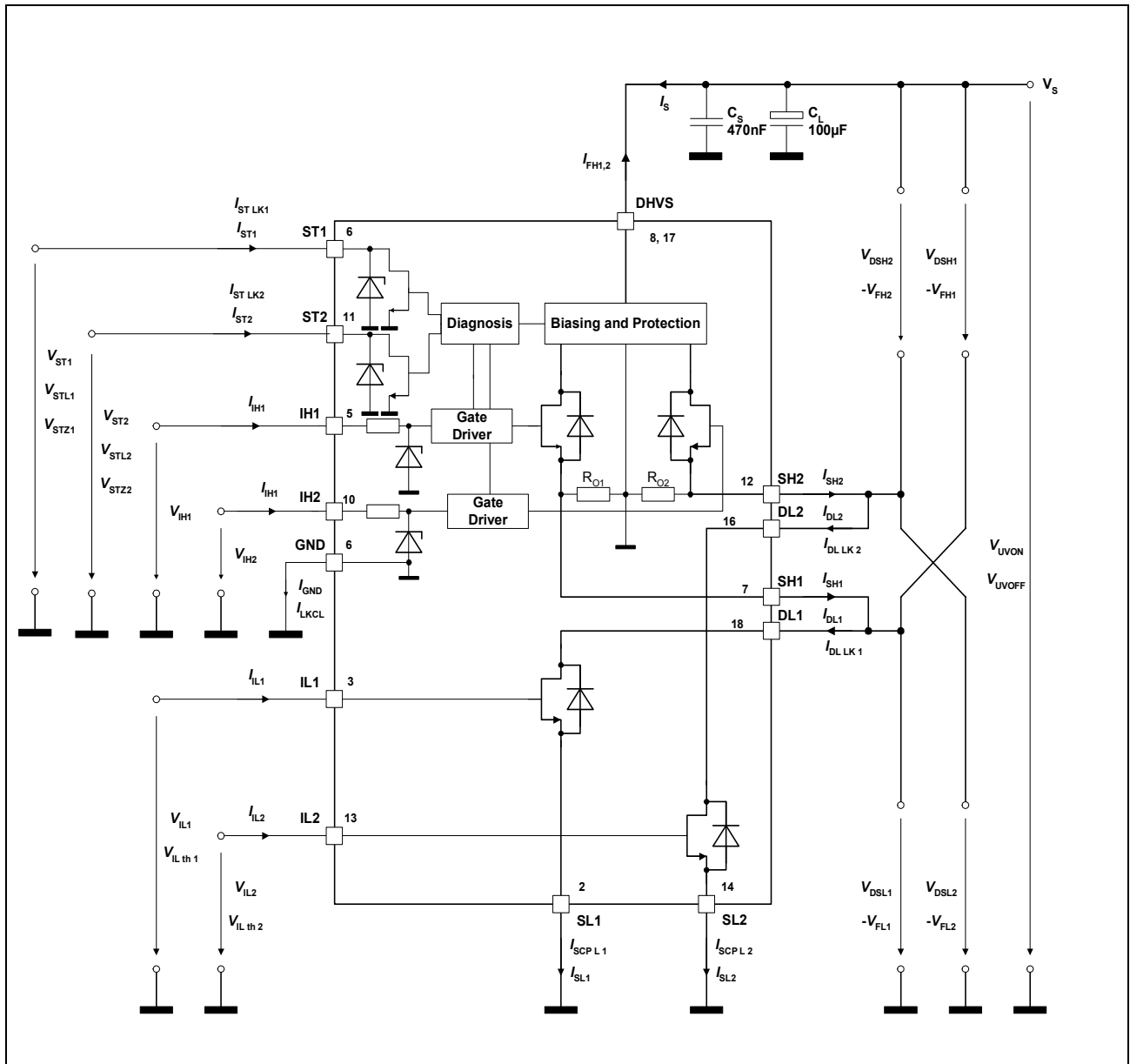
Figure 3 Test Circuit
