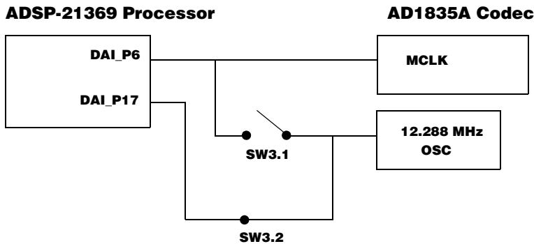
Figure 2-5. Audio Clock Routing
