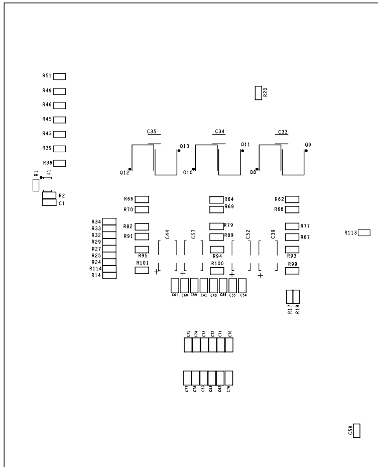
FIGURE 8. BOTTOM SILKSCREEN
