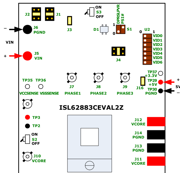
FIGURE 1. TEST SET-UP
