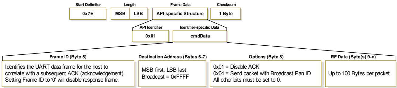
Figure 23: TX Packet (16-bit address) frames
