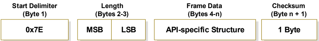
Figure 12: UART data frame structure:
