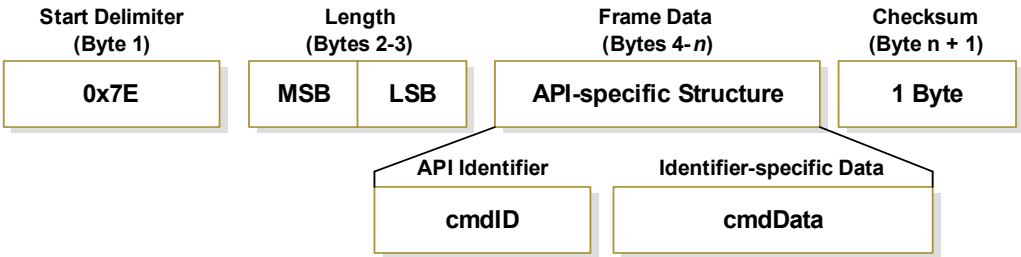
Figure 14: UART Data Frame and API-specific Structure:
