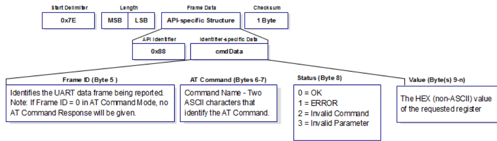
Figure 19: AT Command response frames
