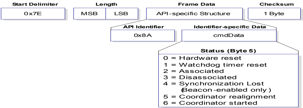
Figure 15: Modem Status frames
