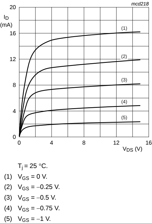
Fig 8. Typical output characteristics; PMBFJ309.
