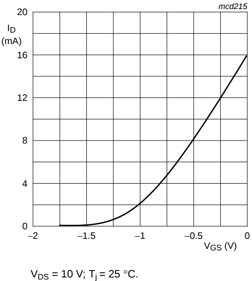
Fig 7. Typical transfer characteristics; PMBFJ308.
