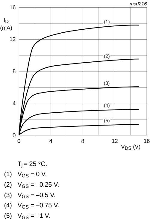
Fig 6. Typical output characteristics; PMBFJ308.
