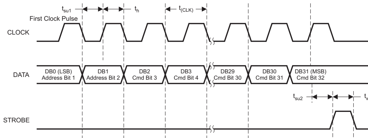
Figure 1. Serial Programming Timing
