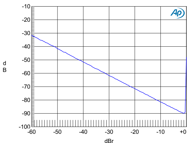
Figure 5-20. THD+N (Relative) vs. Level, Preamp Setting: 0 dB, PGA Setting: 0 dB, 1 kHz
