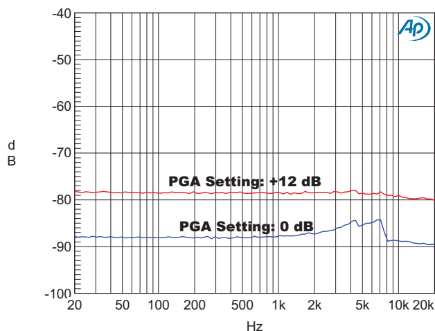
Figure 5-18. THD+N (Relative) vs. Frequency, Preamp Setting: +10 dB, -1 dBFS
