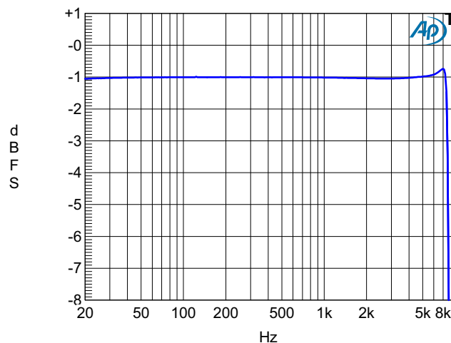
Figure 5-16. Frequency Response, FS_{ext} = 8 kHz, Notch Filter Enabled, Preamp Enabled (+10 or +20 dB), -1 dBFS
