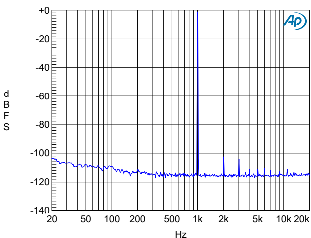
Figure 5-4. Output FFT, Preamp Setting: +10 dB, PGA Setting: +12 dB, 1 kHz, -1 dBFS
