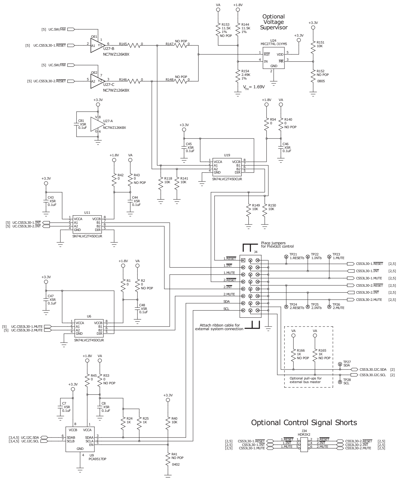
Figure 6-7. Level Shifters, Control I/O Header
