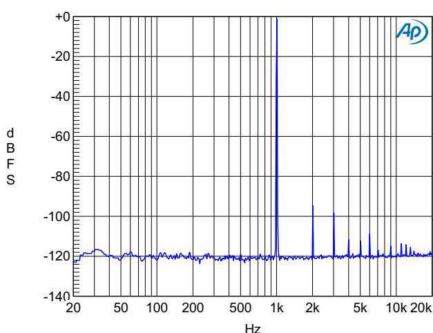
Figure 5-2. Output FFT, Preamp Setting: 0 dB, PGA Setting: +12 dB, 1 kHz, -1 dBFS
