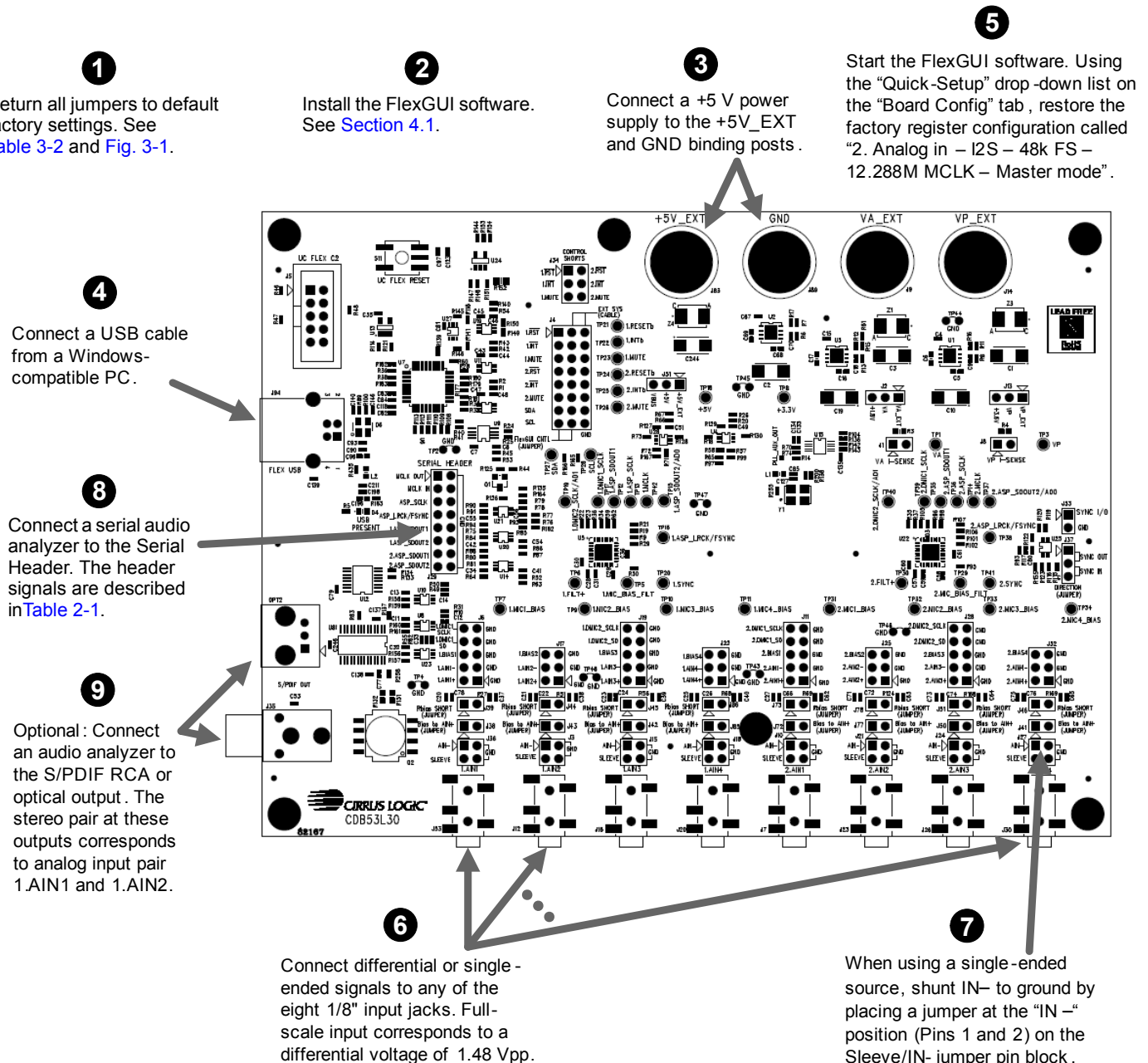
Figure 2-1. CDB53L30 Factory Default Jumper Settings
