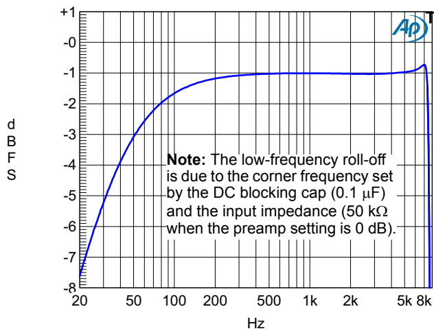
Figure 5-14. Frequency Response, FS_{ext} = 8 kHz, Notch Filter Enabled, Preamp Bypassed (0 dB), -1 dBFS
