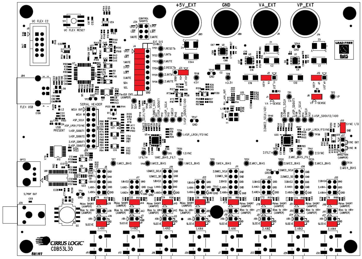
Figure 3-1. CDB53L30 Factory Default Jumper Settings
