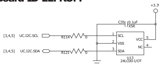
Figure 6-6. Microcontroller
