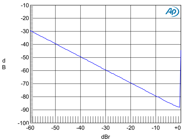
Figure 5-22. THD+N (Relative) vs. Level, Preamp Setting: +10 dB, PGA Setting: 0 dB, 1 kHz
