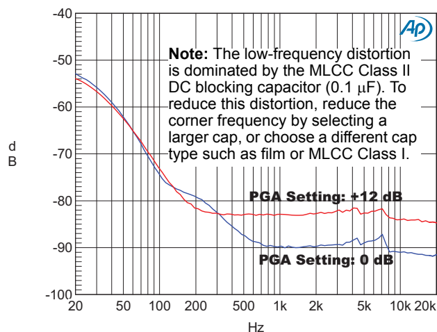
Figure 5-17. THD+N (Relative) vs. Frequency, Preamp Setting: 0 dB, -1 dBFS
