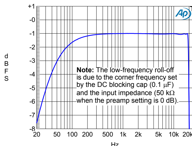
Figure 5-10. Frequency Response, Notch Filter Enabled, Preamp Bypassed (0 dB), -1 dBFS
