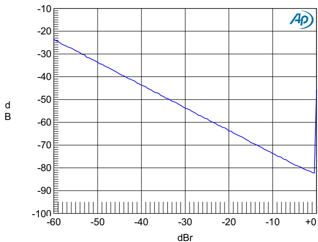
Figure 5-24. THD+N (Relative) vs. Level, Preamp Setting: +20 dB, PGA Setting: 0 dB, 1 kHz
