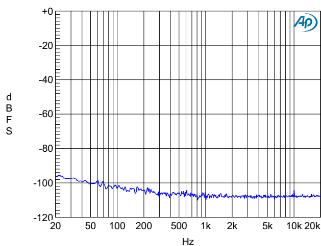
Figure 5-26. FFT, Adjacent Channel Crosstalk at 10 kHz, Preamp Setting: +20 dB, PGA Setting: +12 dB, -1 dBFS
