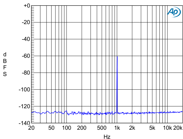
Figure 5-7. Output FFT, 1 kHz, -60 dBFS
