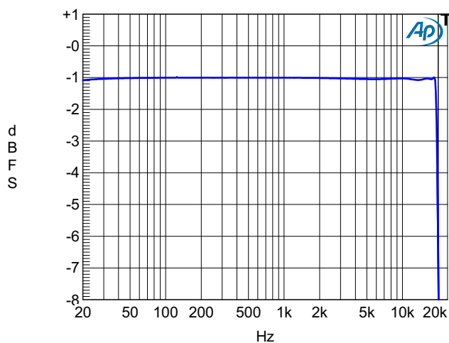
Figure 5-12. Frequency Response, Notch Filter Enabled, Preamp Enabled (+10 or +20 dB), -1 dBFS
