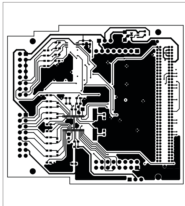
Figure 5. MAXSPCSPARTAN6+ PCB Layout—Solder Side
