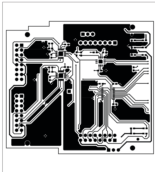
Figure 4. MAXSPCSPARTAN6+ PCB Layout—Component Side
