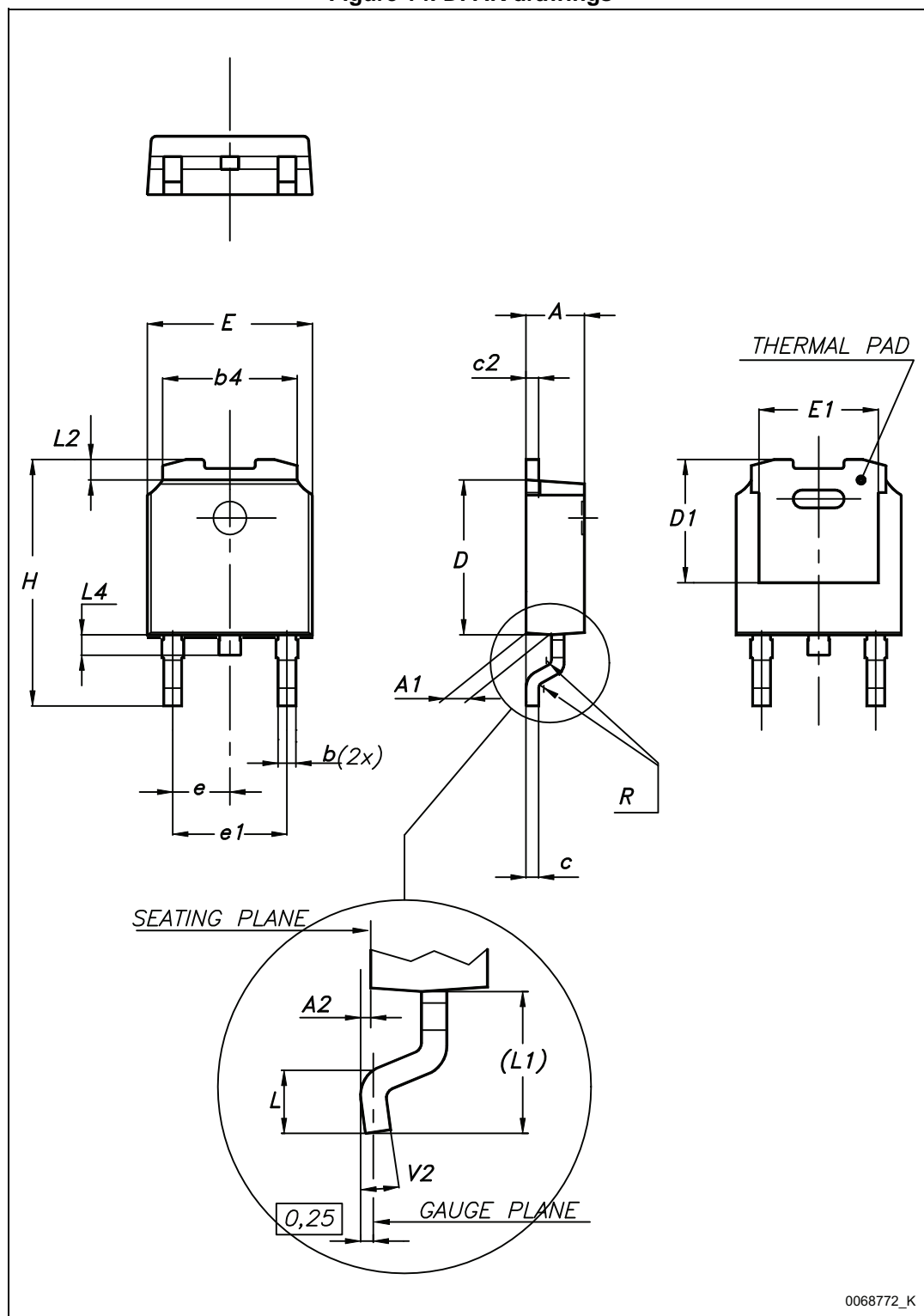
Figure 14. DPAK drawings
