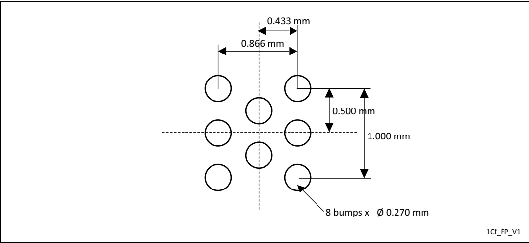
Figure 19. M24512-DFCS6TP/K recommended footprint
