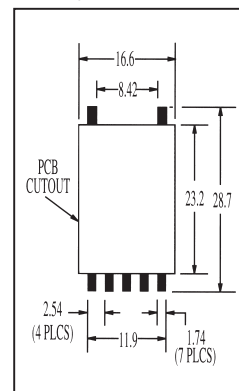
Pad Layout D
