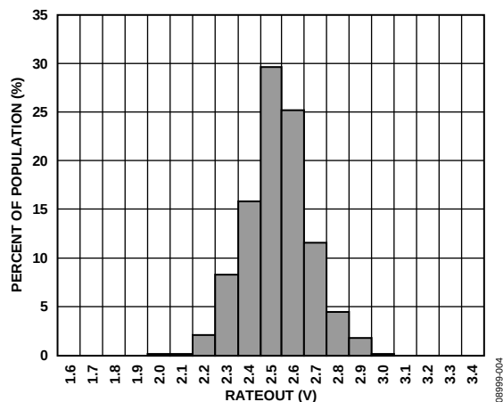
Figure 4. Null Output at 25°C ( V_{\text{RATIO}} = 5 \text{ V} )
