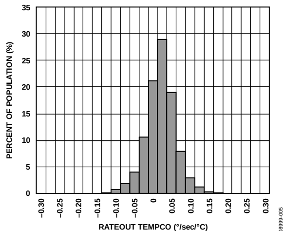
Figure 5. Null Drift over Temperature ( V_{\text{RATIO}} = 5 \text{ V} )
