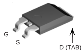
PLUS220SMD (IXTV...S)
