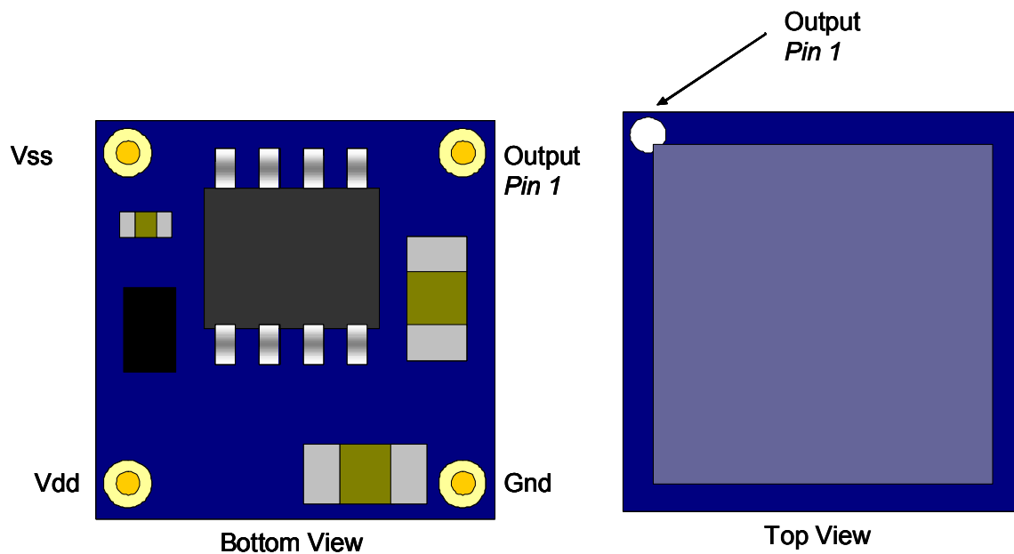
Fig. 4 Pin Assignment for the PS25205B
