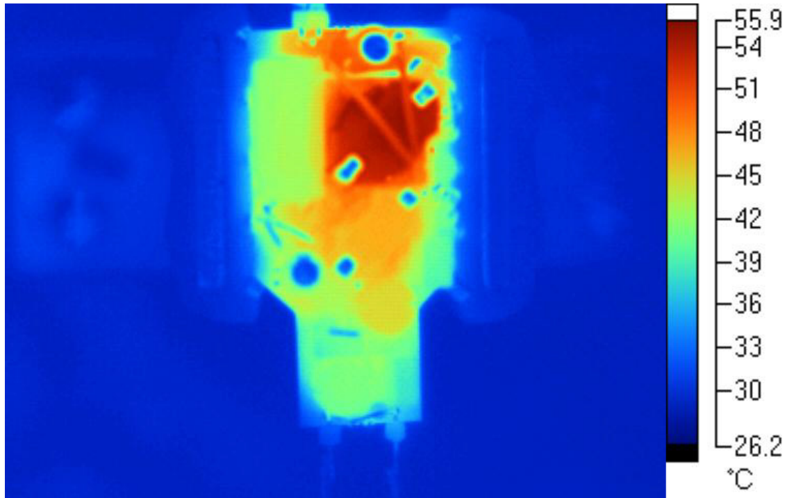
Figure 8. Top Thermal
