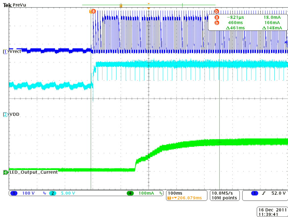
Figure 22. ILED at Medium Dim Angle, Turn-on Waveforms
