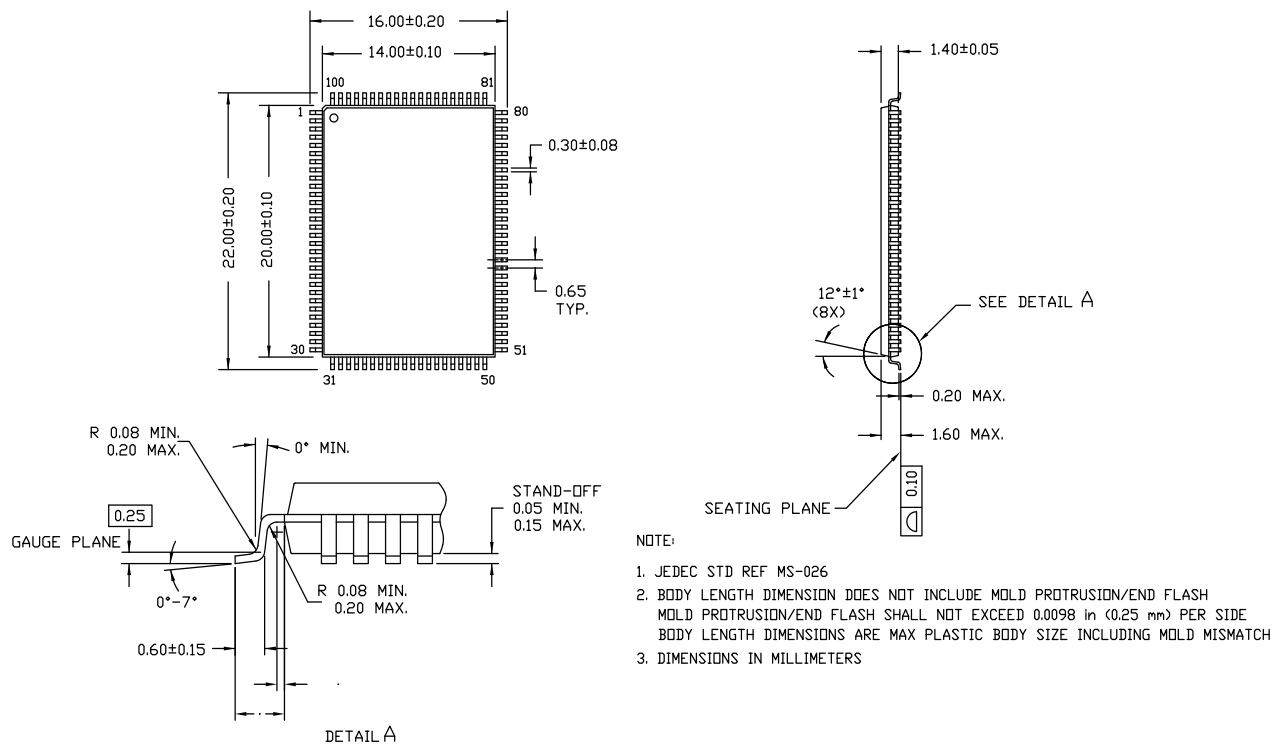
Figure 9. 100-pin TQFP (14 × 20 × 1.4 mm) A100RA Package Outline, 51-85050
