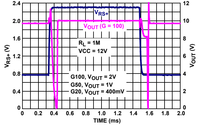
FIGURE 6. V_{OUT} vs V_{RS+} , V_{SENSE} = 20mV TRANSIENT RESPONSE
