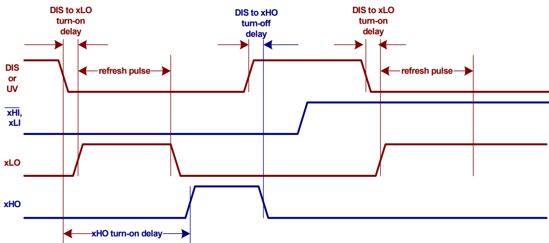
FIGURE 5. DISABLE FUNCTION
