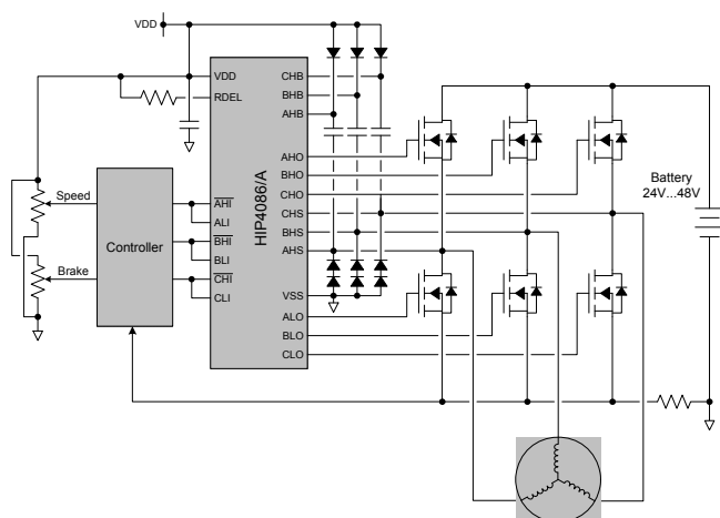
FIGURE 1. TYPICAL APPLICATION
