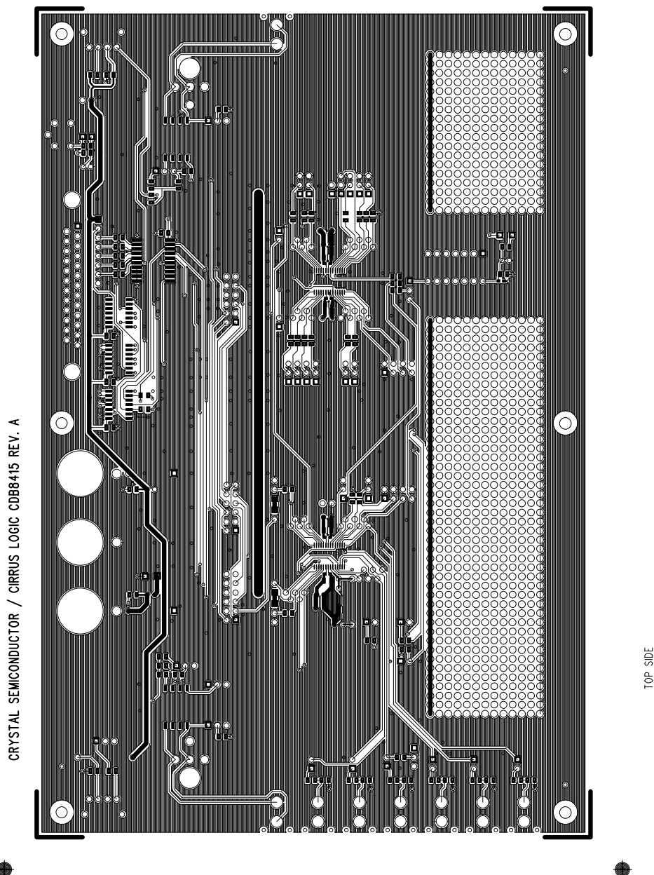
Figure 10. Top PCB
