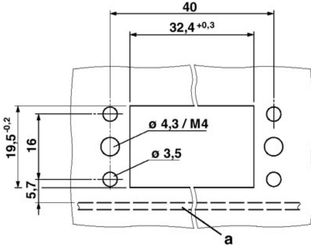
Dimensioned drawing
