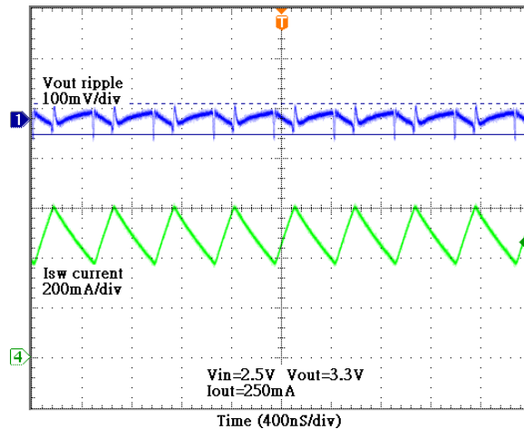
Fig. 20 Switching Current vs. Output Ripple
