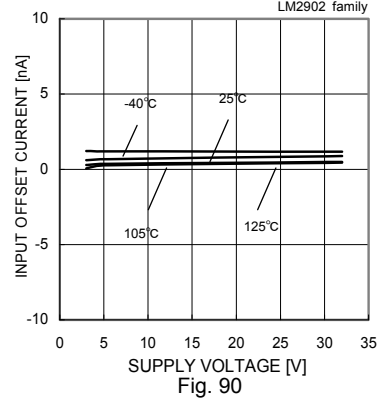
Fig. 90 Input Offset Current – Supply Voltage (Vicm=0[V], VOUT=1.4[V])
