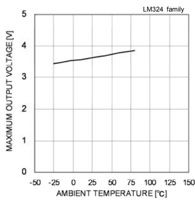
Fig. 29 Maximum Output Voltage - Ambient Temperature (VCC=5[V], RL=2[kΩ])
