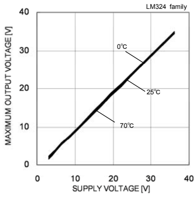
Fig. 28 Maximum Output Voltage - Supply Voltage (RL=10[kΩ])
