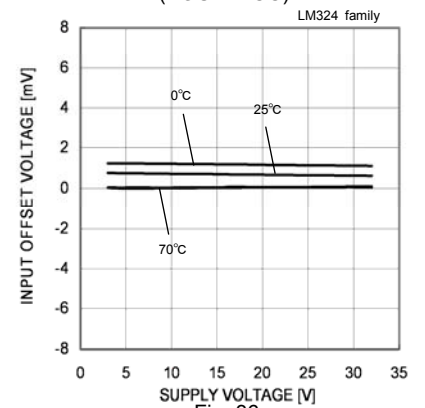
Fig. 36 Input Offset Voltage - Supply Voltage (Vicm=0[V], VOUT=1.4[V])
