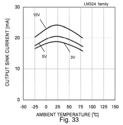
Fig. 33 Output Sink Current - Ambient Temperature (VOUT=VCC)
