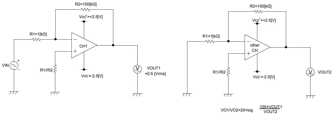
Fig.101 Measurement Circuit3
