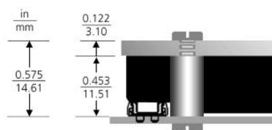
Figure 15-3 — Slotted baseplate; Height above board with standoff
