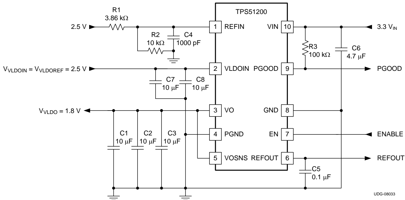
Figure 29. 3.3-V IN , LDO Configuration
