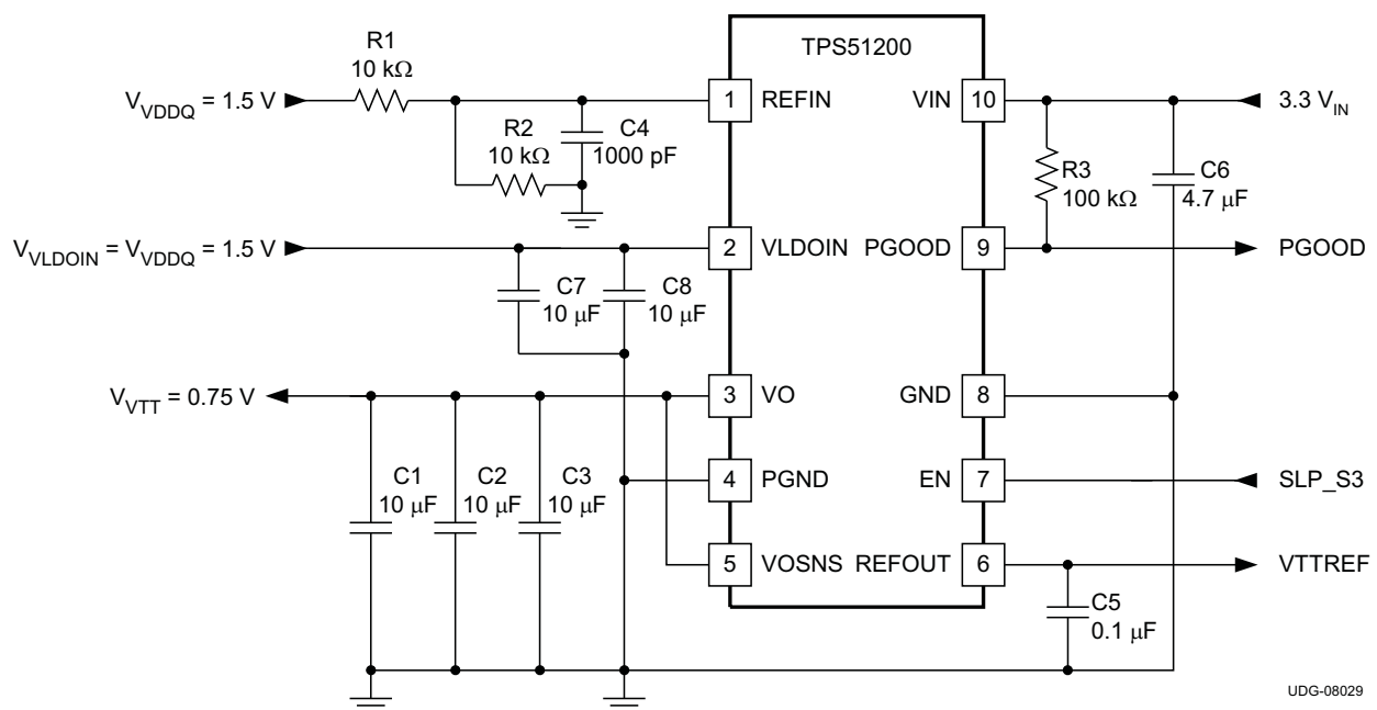
Figure 21. 3.3- V_{IN} , DDR3 Configuration
