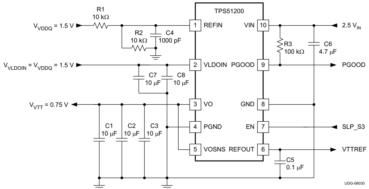
Figure 26. 2.5-V IN , DDR3 Configuration
