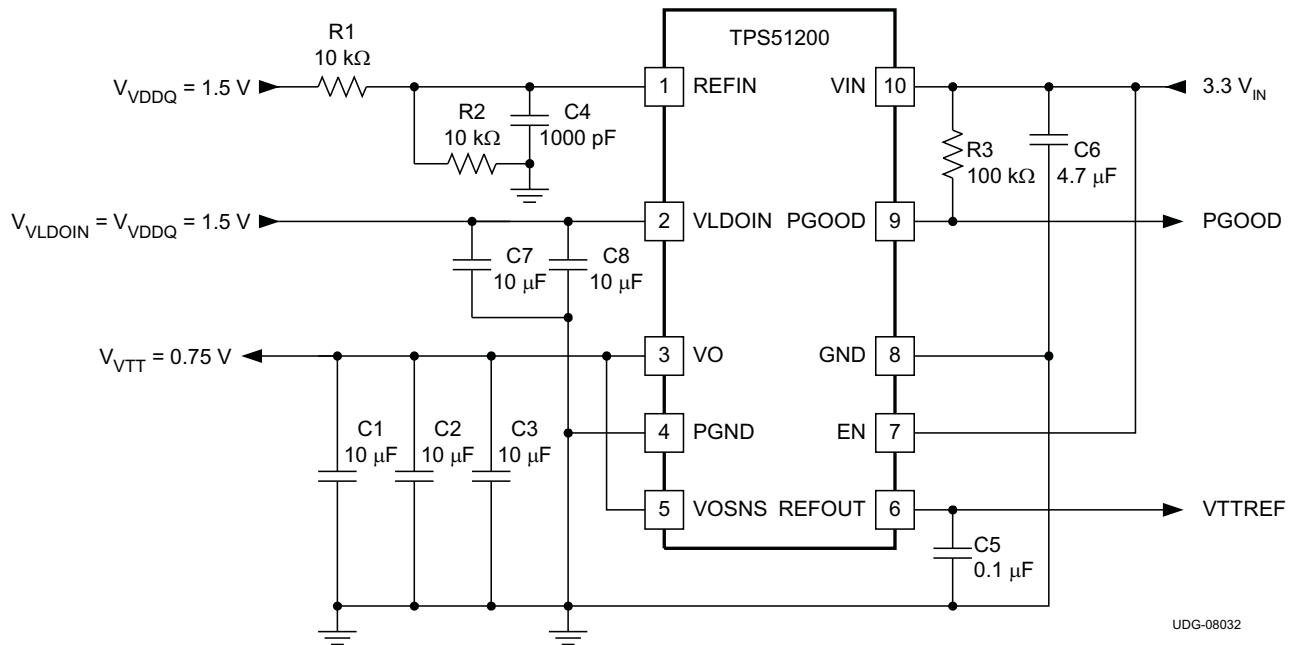
Figure 28. 3.3- V_{IN} , DDR3 Tracking Configuration
