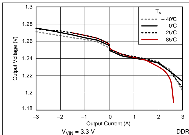
Figure 1. Load Regulation
