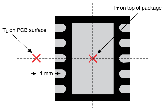
Figure 33. Package Thermal Measurement
