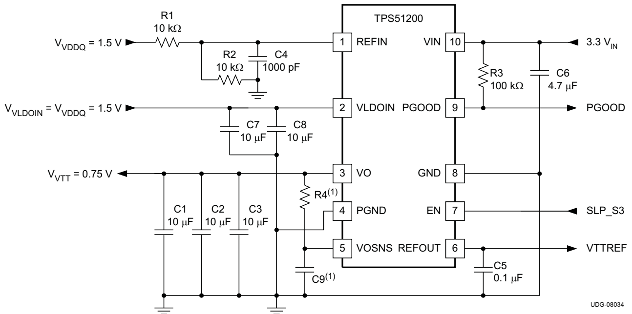
Figure 30. 3.3-V IN , DDR3 Configuration with LFP
