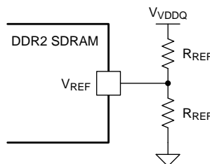
Figure 20. Resistor Divider Circuit
