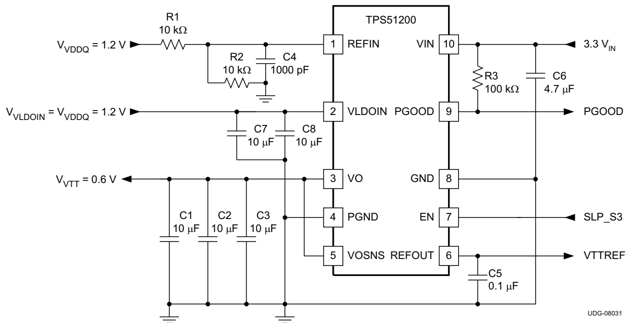
Figure 27. 3.3-V IN , LP DDR3 or DDR4 Configuration
