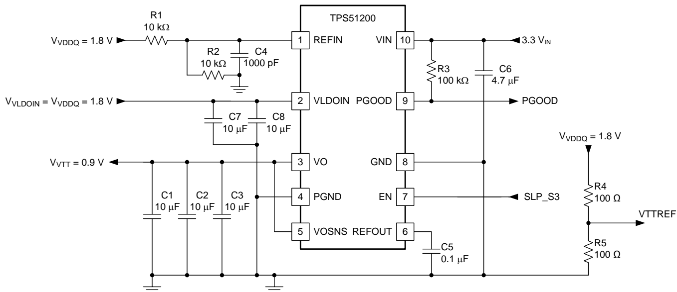
Figure 25. 3.3- V_{IN} , DDR2 Configuration
