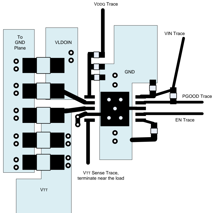
Figure 31. Layout Recommendation
