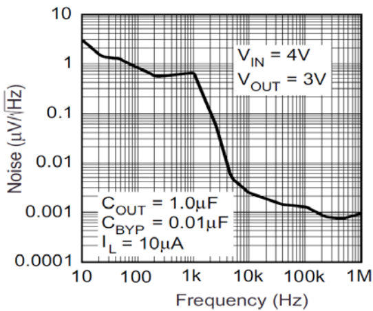
Figure 13. Noise Performance
