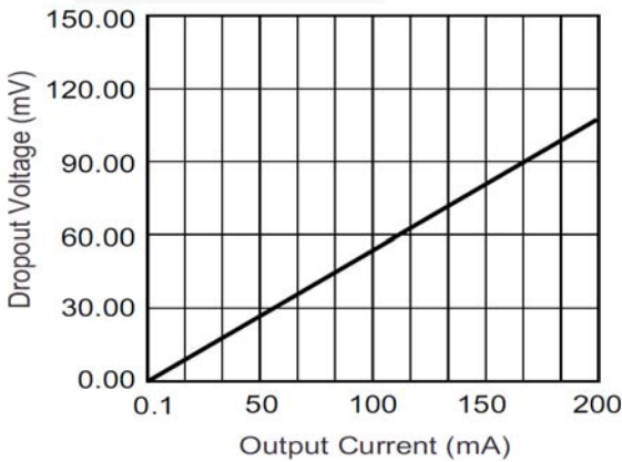
Figure 19. Dropout Voltage
