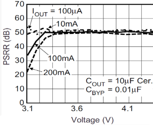
Figure 12. PSRR vs. Voltage Drop
