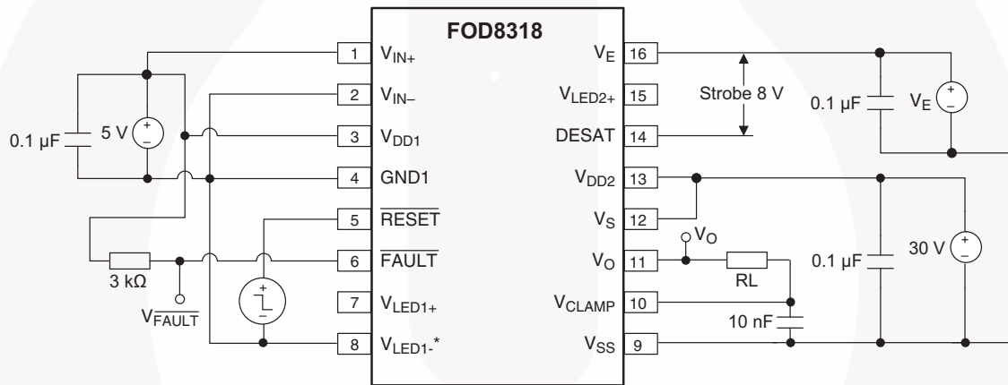
Figure 44. DESAT Sense ( t_{DESAT(90\%)} , t_{DESAT(10\%)} ), DESAT Fault ( t_{DESAT(FAULT)} ), and ( t_{DESAT(LOW)} ) Test Circuit
