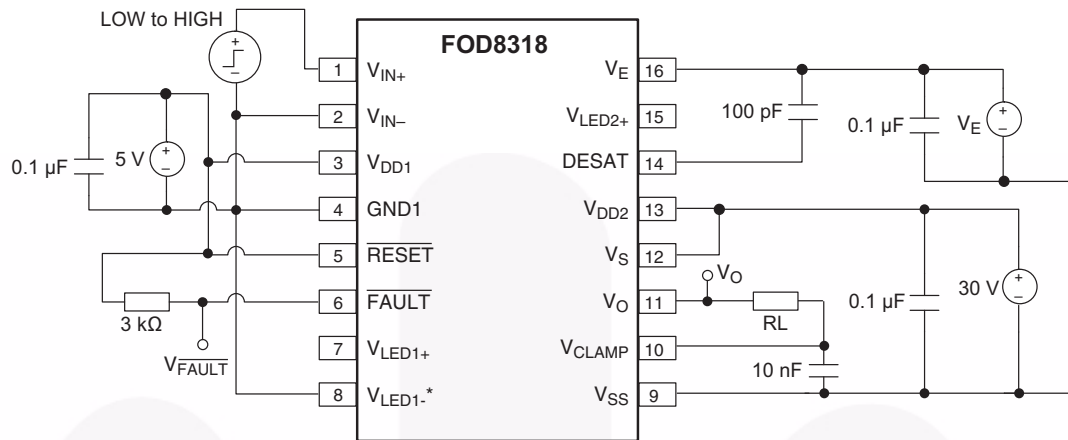
Figure 44. DESAT Sense ( t_{DESAT(90\%)} , t_{DESAT(10\%)} ), DESAT Fault ( t_{DESAT(FAULT)} ), and ( t_{DESAT(LOW)} ) Test Circuit
