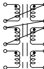
Figure 7 Turns ratio: 4:1:1
