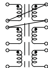
Figure 8 Turns ratio: 3:1:1:1
