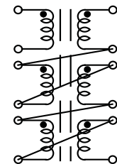
Figure 3 Turns ratio: 1:5 or 5:1
