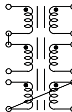
Figure 2 Turns ratio: 1:1:1
