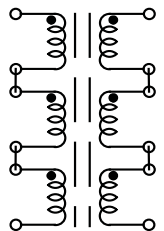
Figure 1 Turns ratio: 1:1
