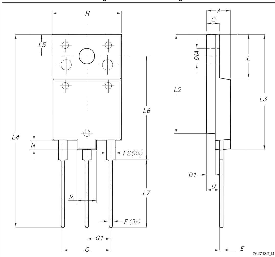
Figure 23. TO-3PF drawing
