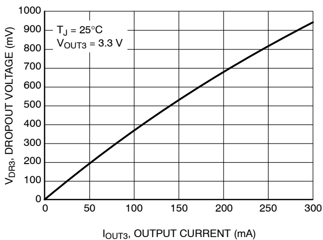
Figure 16. Dropout LDO3 vs Output Current
