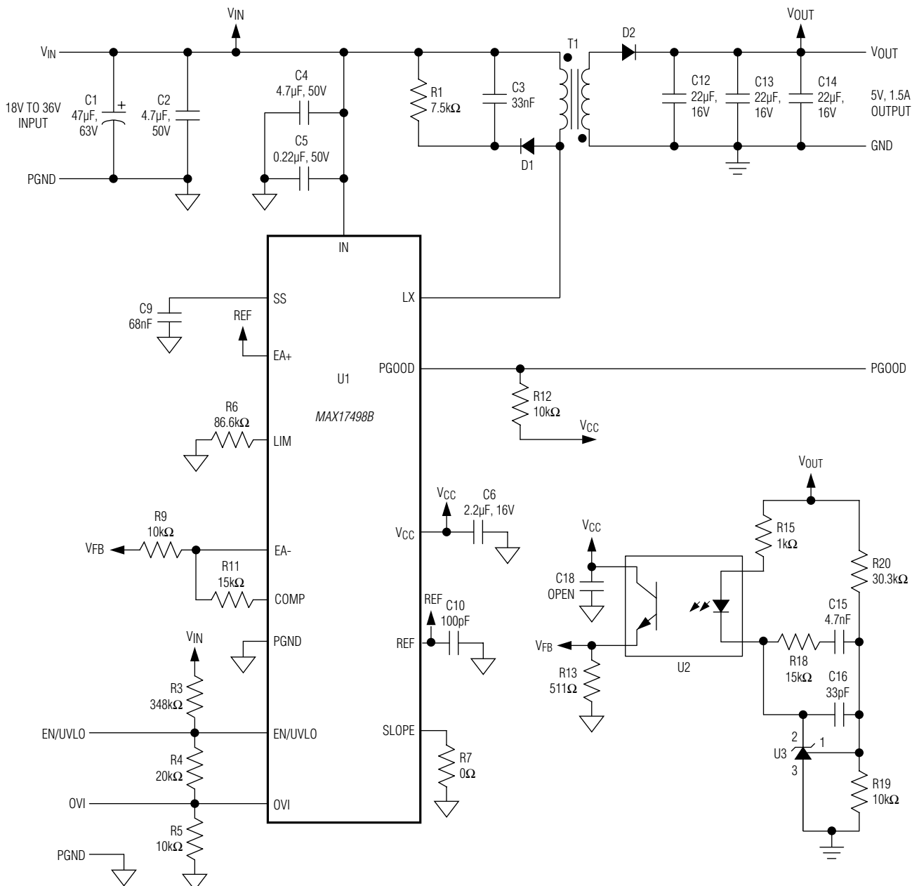
Figure 10. MAX17498B Isolated DC-DC Power Supply
