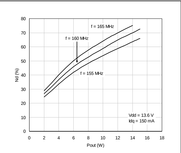
Figure 8. Efficiency vs P_{OUT} and frequency @ V_{DD} = 13.6\text{ V}
