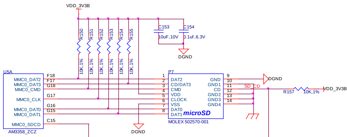
Figure 36. microSD Design
