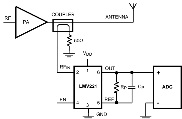
Figure 2. LMV221 with feedback (R)C Low Pass Filter
