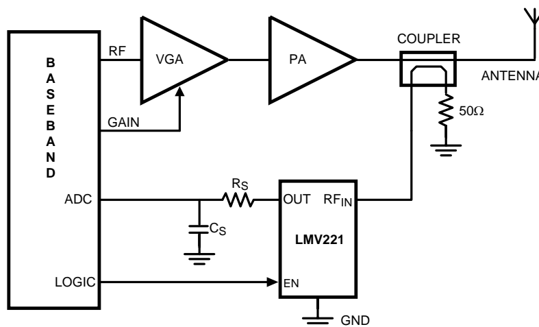
Figure 72. Transmit Power Control System
