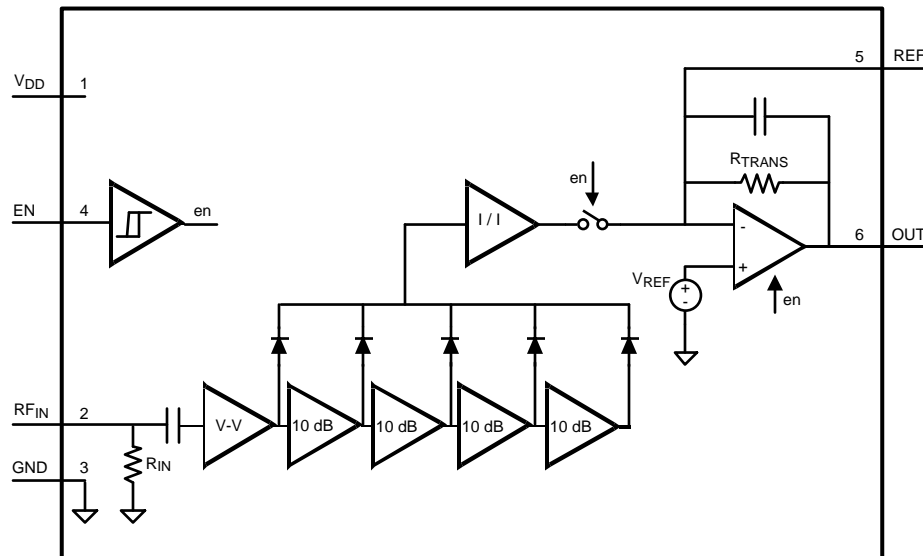
Figure 80. Block Diagram of the LMV221
