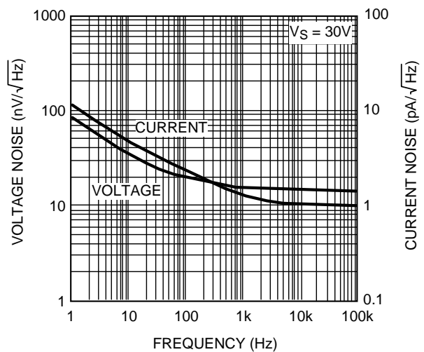
Figure 42. Input-Referred Noise Density vs Frequency
