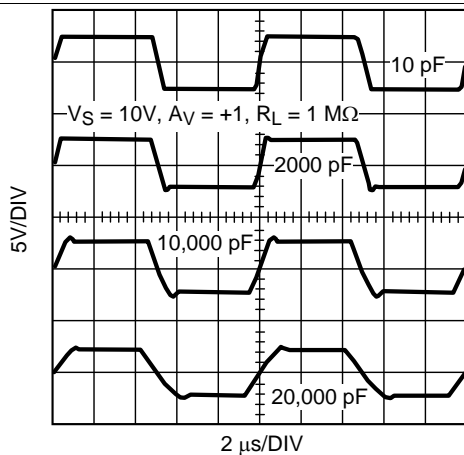
Figure 39. Large Signal Step Response for Various Capacitive Loads
