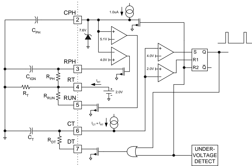
Figure 6: Oscillator section block diagram with external component connection
