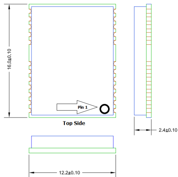
Figure 2 – Mechanical Layout
