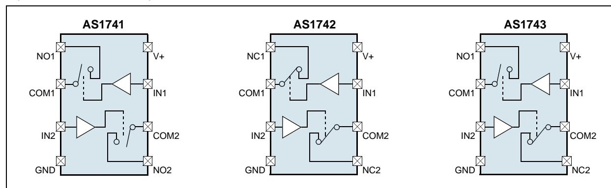
Figure 1. MSOP Block Diagrams
