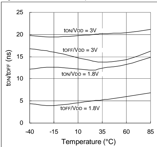
Figure 9. t ON /t OFF vs. Temperature
