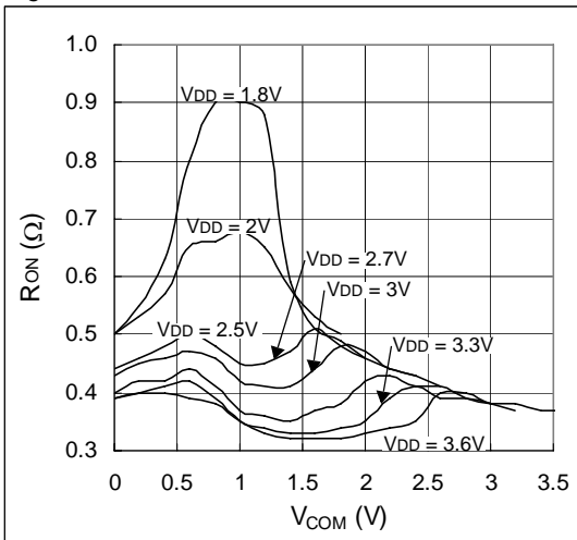
Figure 7. R ON vs. V COM
