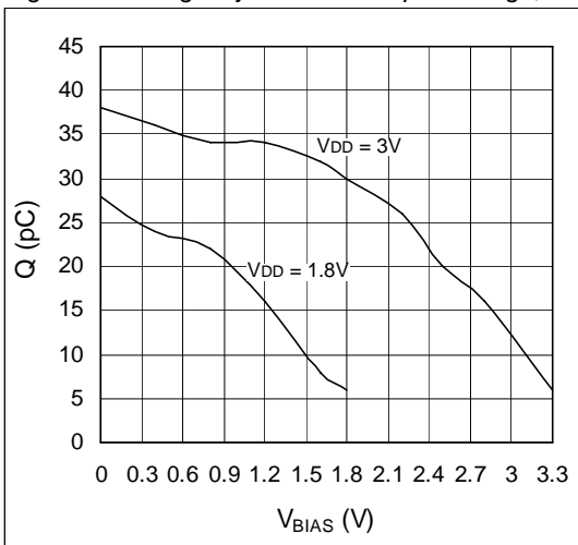
Figure 5. Charge Injection vs. Output Voltage; MSOP
