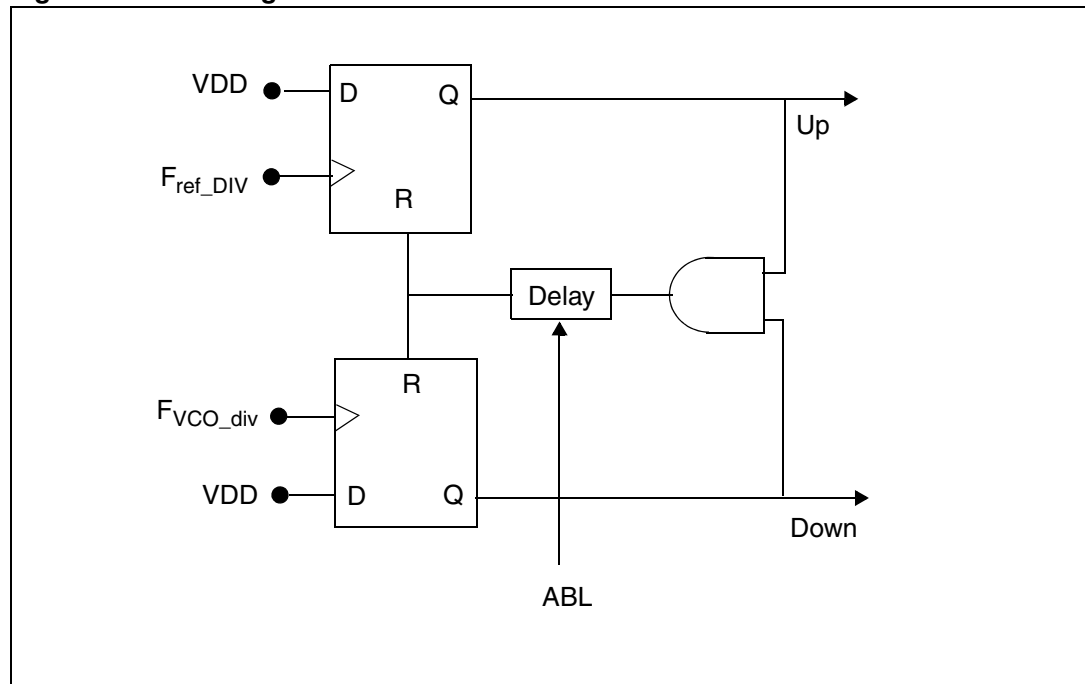
Figure 11. PFD diagram
