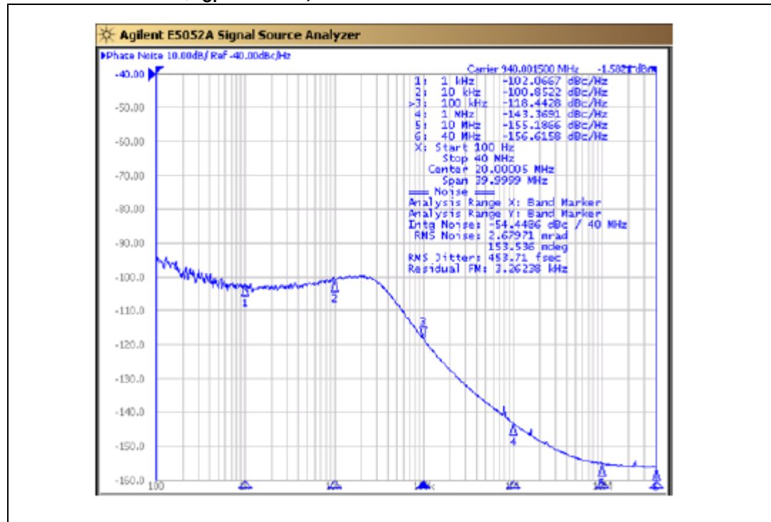
Figure 7. LOA (VCOA div. by 4) closed-loop phase noise at 0.94 GHz ( F_{\text{STEP}} = 200 \text{ kHz} , I_{\text{CP}} = 1.5 \text{ mA} )
