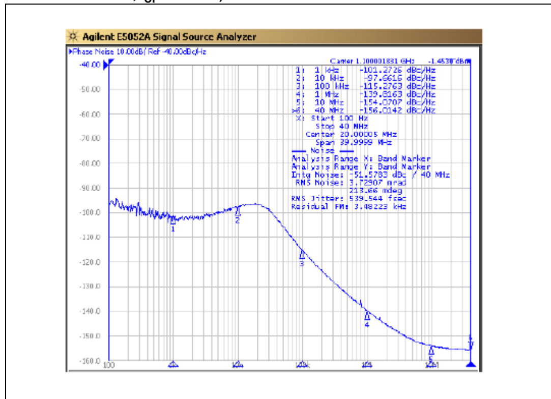
Figure 8. LOB (VCOB div. by 4) closed-loop phase noise at 1.1 GHz ( F_{\text{STEP}} = 200 \text{ kHz} , I_{\text{CP}} = 1.5 \text{ mA} )
