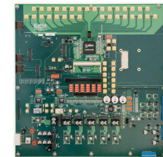
LatticeSC Communications Evaluation Board
