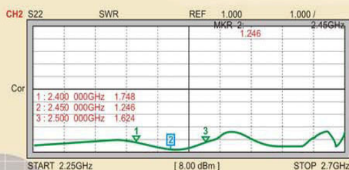
SWR
