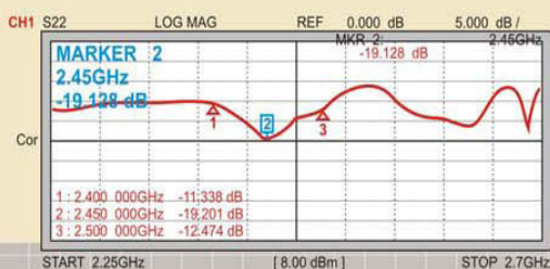
Return Loss
