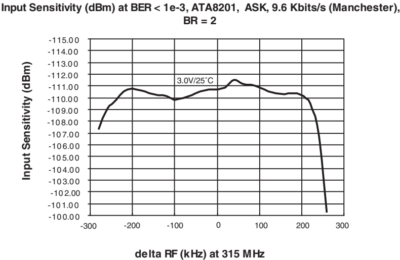
Figure 2-3. Measured Sensitivity (315MHz, ASK, 9.6Kbits/s, Manchester) Versus Frequency Offset
