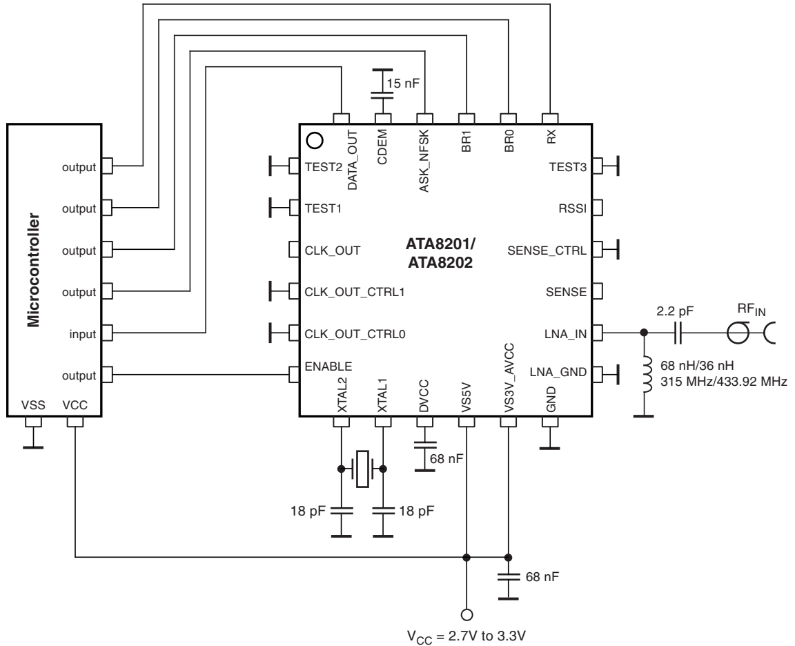
Figure 9-1. 3V Application
