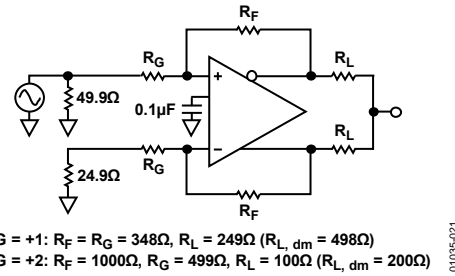
Figure 59. Test Circuit for Output Balance
