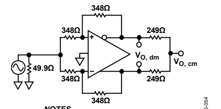
Figure 61. CMRR Test Circuit
