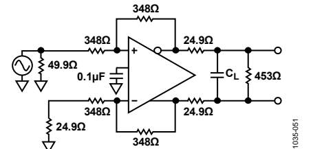
Figure 60. Test Circuit for Capacitor Load Drive
