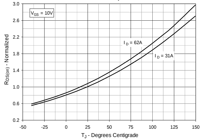
Fig. 4. R_{DS(on)} Normalized to I_D = 31A Value vs. Junction Temperature
