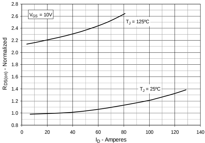
Fig. 5. R_{DS(on)} Normalized to I_D = 31A Value vs. Drain Current
