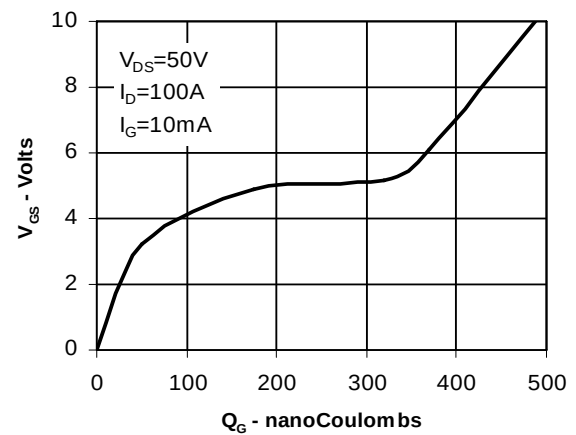
Fig. 10. Gate Charge
