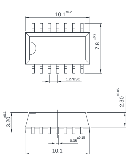
External dimensions
