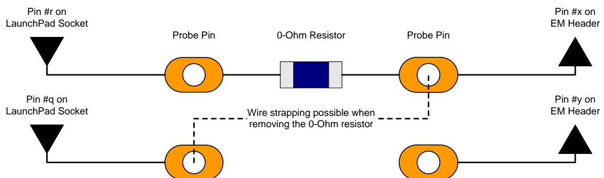
Figure 3 - Re-wiring Concept
