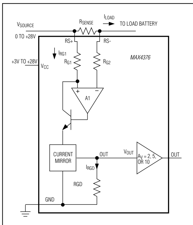
Figure 1. Functional Diagram
