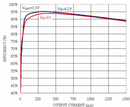
Fig. 4: Efficiency vs Output Current V_{OUT}=3.3V
