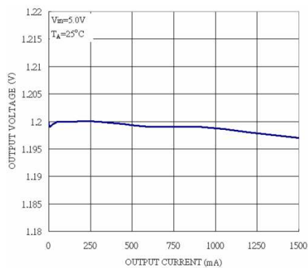
Fig. 9: Output Voltage vs Load Current
