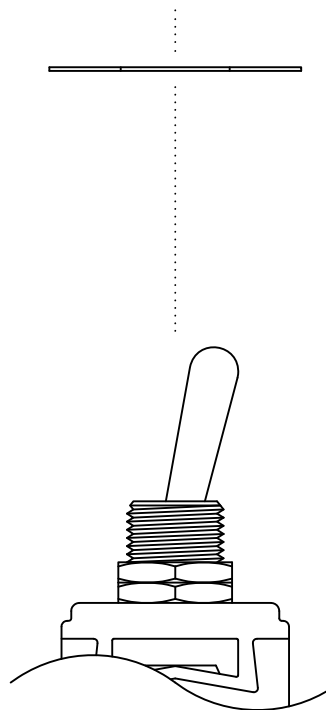
EXPLODED VIEW
