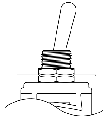
ASSEMBLED VIEW
