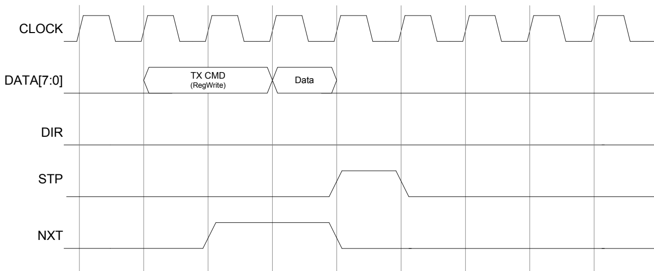
Figure 11. Register Write
