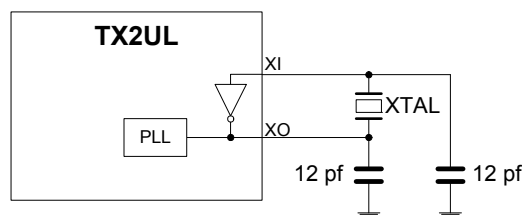
Figure 2. Crystal Configuration
